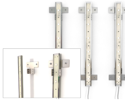
Heavy duty bracket - Part no. BGT-PT-060 For installation where fixture security is critical
