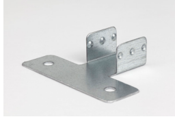
Install clips/rail
