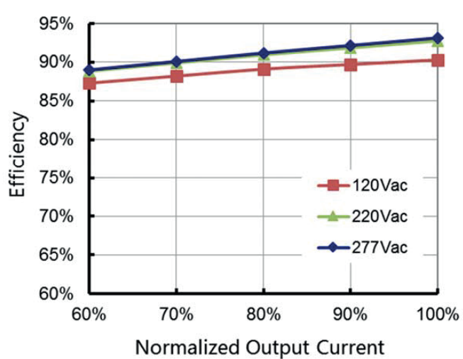
Efficiency vs. Load (24V Model)
