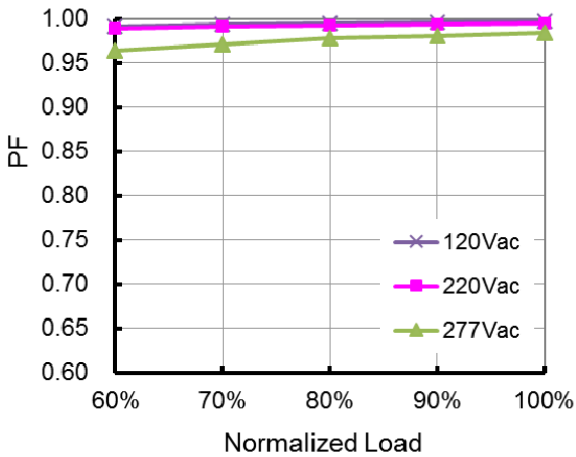
Power Factor vs. Load
