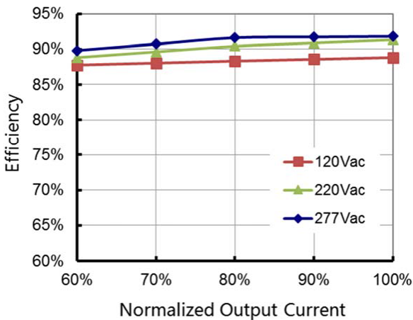
Efficiency vs. Load (24V Model)
