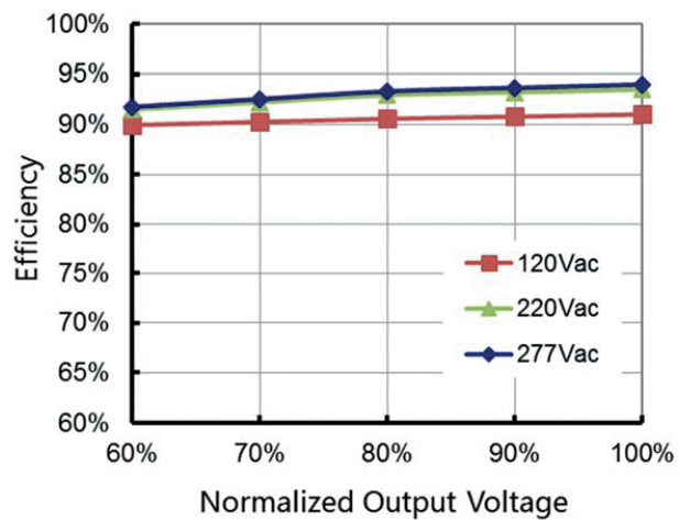
Efficiency vs. Load (1.4A Model)
