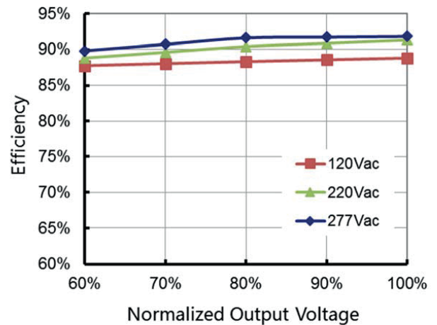
Efficiency vs. Load (1.4A Model)
