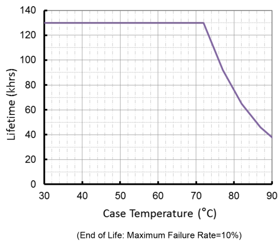
Lifetime vs. Case Temperature
