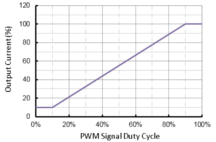
PWM Dimming Curve
