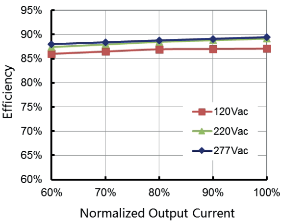
Efficiency vs. Load (24V Model)
