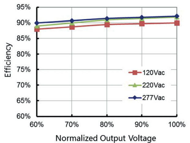
Efficiency vs. Load (1.05A Model)
