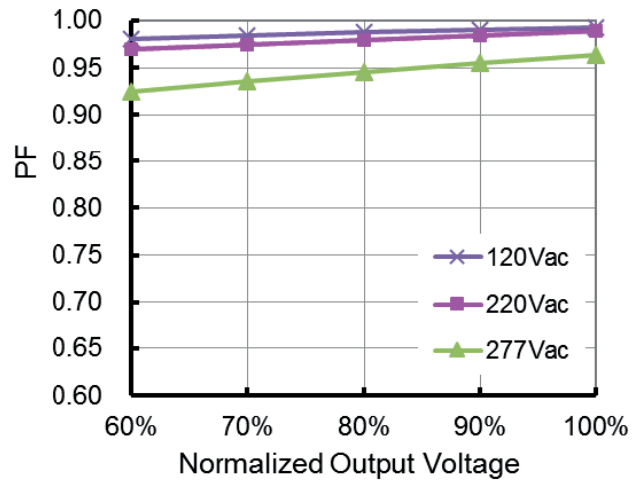
Power Factor vs. Load
