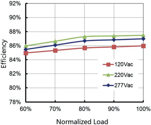
Efficiency vs. Load (24V Model)
