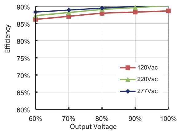
Efficiency vs. Load (1.05A Model)
