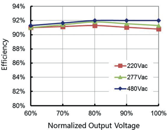
Efficiency vs. Load (2.1A Model)
